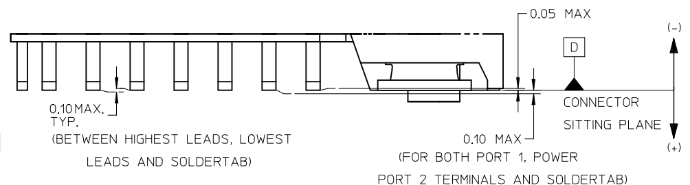
DETAIL 1
