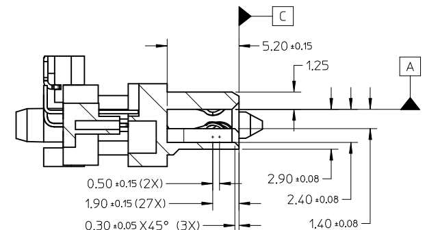
SECTION Z-Z
