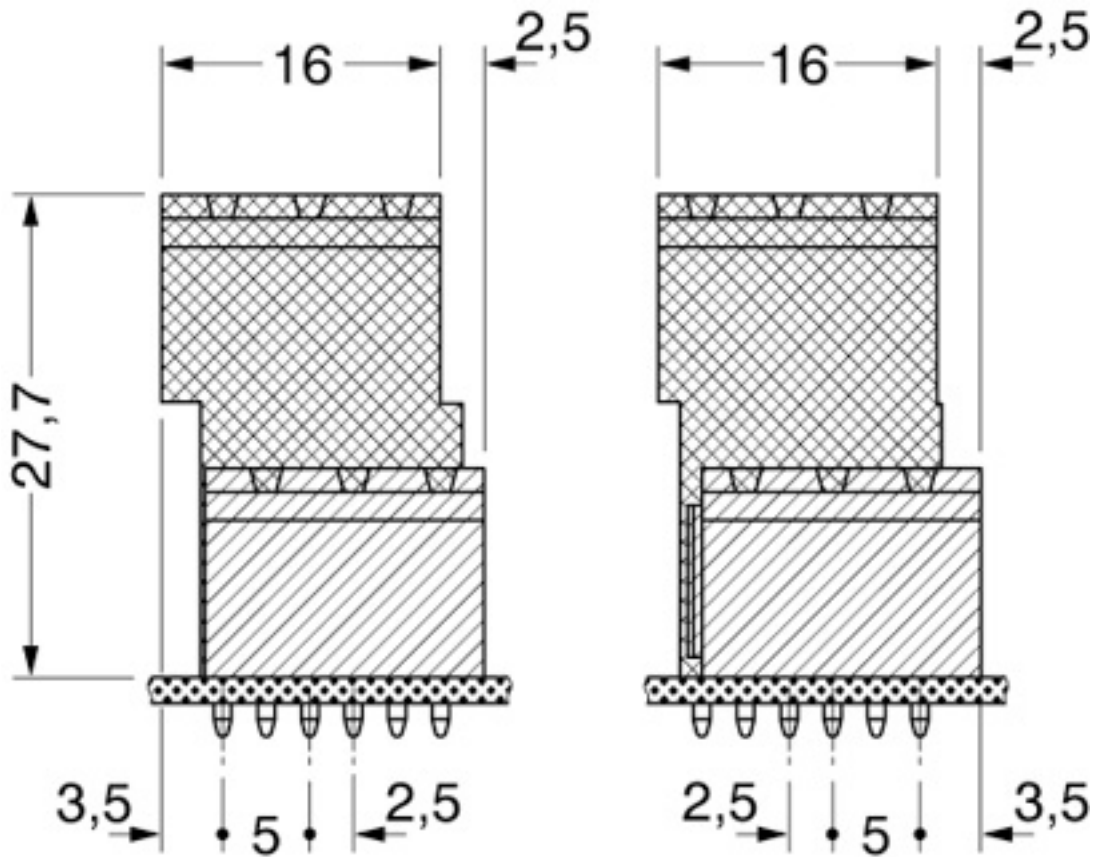
Dimensioned drawing
