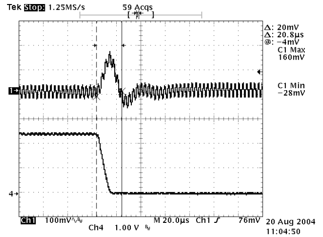
Figure 22: Typical transient response to step load change at 0.5A/μS from 50% to 0% of Io, max at 5.0Vin, 2.5V out (measurement with a 1uF ceramic and a 10μF tantalum)
