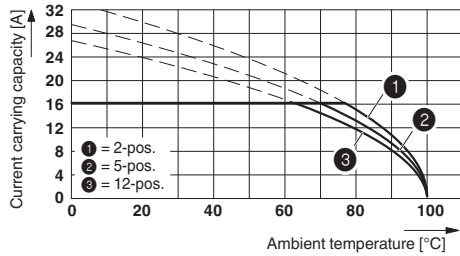
Derating curve for: MSTB 2,5 HC/14-ST with MSTBA 2,5 HC/14-ST-5,08-G
