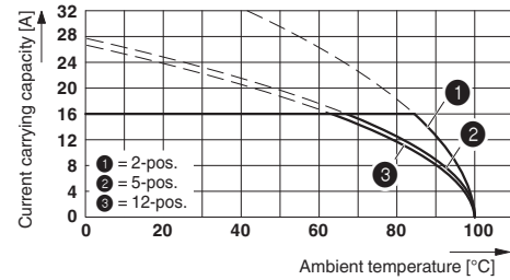
Derating curve for: MSTB 2,5 HC/14-ST-5,08 with MSTBVA 2,5 HC/14-ST-5,08-G
