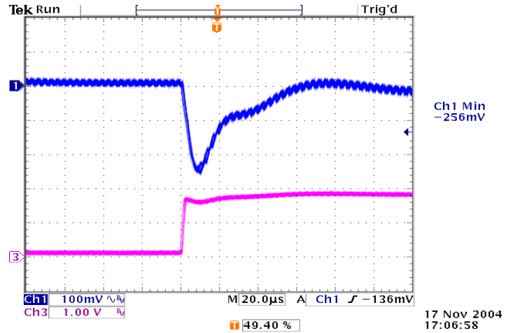
Figure 26: Typical transient response to step load change at 2.5A/µS from 50% to 100% of I_o , max at 3.3Vin, 1.8V out (Cout = ceramic, 10µF tantalum)
