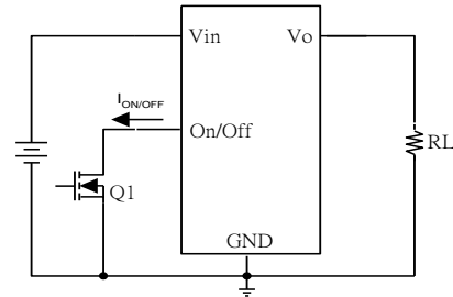
Figure 34: Positive remote On/Off implementation
