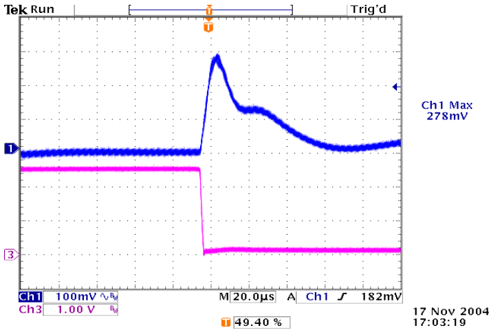
Figure 23: Typical transient response to step load change at 2.5A/µS from 100% to 50% of I_o , max at 3.3Vin, 2.5V out (Cout = ceramic, 10µF tantalum)
