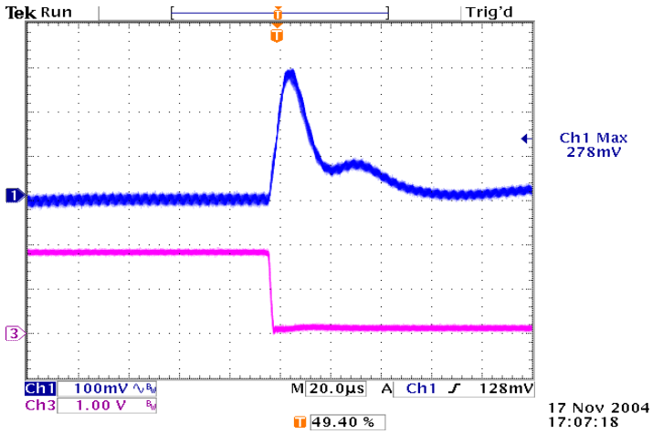
Figure 25: Typical transient response to step load change at 2.5A/µS from 100% to 50% of I_o , max at 3.3Vin, 1.8V out (Cout = ceramic, 10µF tantalum)
