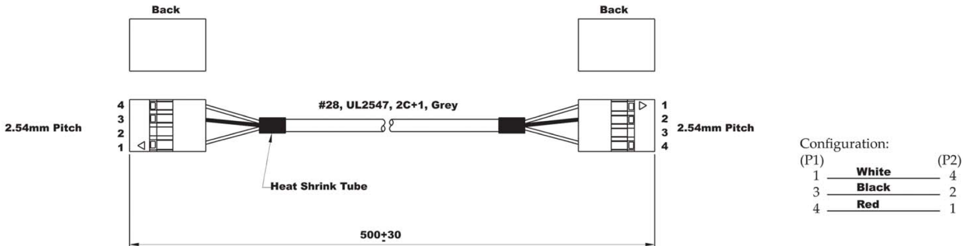
AK2525-R (4-Pin, Female, 2.54mm to 4-Pin, Female, 2.54mm...UL2547 Cable, 3-Wire)
