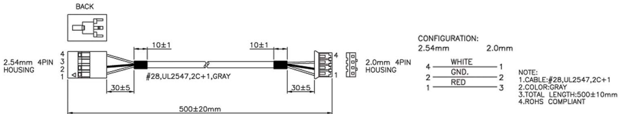
AK2524-R (4-Pin, Female, 2mm to 4-Pin, Female, 2.54mm...UL2547 Cable, 3-Wire)
