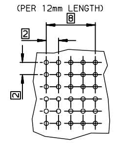
LAYOUT FOR P.C.B
