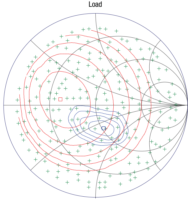
Figure 20. Load Pull, @ 5 V and 95 mA
